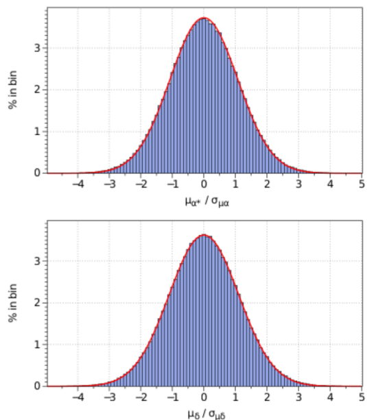
Fig. 10. Distributions of the normalised components of proper motions of the QSOs found with Gaia data, with \mu_{\alpha^*} (top) and \mu_\delta (bottom). A normal distribution with zero mean and standard deviation of 1.09 for \mu_{\alpha^*} (1.11 for \mu_\delta ) is drawn in red.
