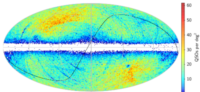
Fig. 1. Sky density per square degree for the quasars of Gaia-CRF2 on an equal-area Hammer–Aitoff projection in Galactic coordinates. The Galactic centre is at the origin of coordinates (centre of the map), Galactic north is up, and Galactic longitude increases from right to left. The solid black line shows the ecliptic. The higher density areas are located around the ecliptic poles.
