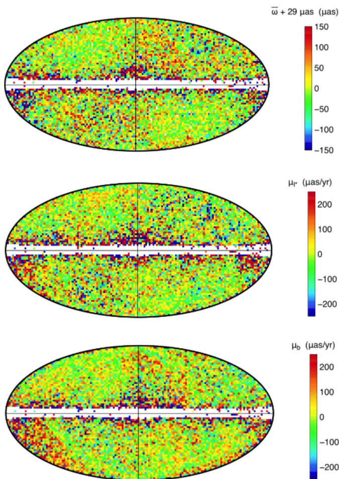
Fig. 11. Spatial distributions (in Galactic coordinates) of the parallaxes and proper motions of the Gaia -CRF2 quasars. From top to bottom: parallax ( \bar{\omega} ), proper motion in Galactic longitude ( \mu_l ), and proper motion in Galactic latitude ( \mu_b ). Median values are computed in cells of approximately 5 \text{ deg}^2 . Maps are in the Hammer–Aitoff projection with Galactic longitude zero at the centre and increasing from right to left.
