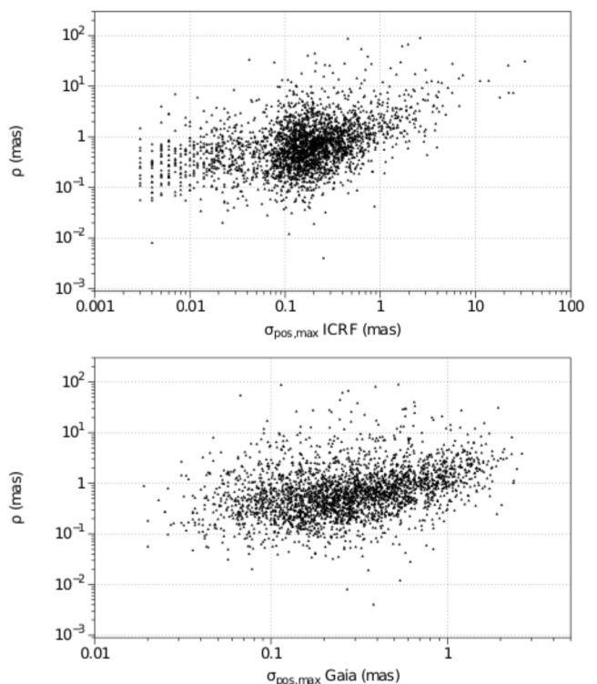
Fig. 17. Angular position differences \rho between Gaia DR2 and the ICRF3-prototype as function of the formal uncertainties \sigma_{pos,max} of the ICRF3-prototype (top) and Gaia DR2 (bottom).
