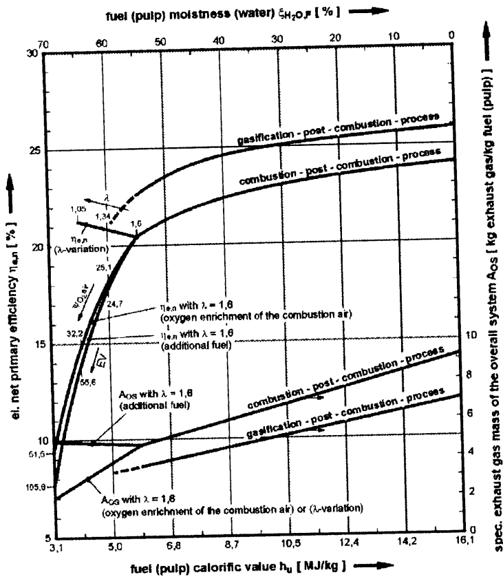
Figure 2: El. net primary efficiency \eta_{e,n} and specific exhaust gas mass A_{OS} dependent upon the fuel (pulp) calorific value h_u and the fuel (pulp) moistness \xi_{H_2O,F} for gasification-post-combustion – processes and combustion-post-combustion – processes by a min. temperature \vartheta_{min} = 950^\circ C .
