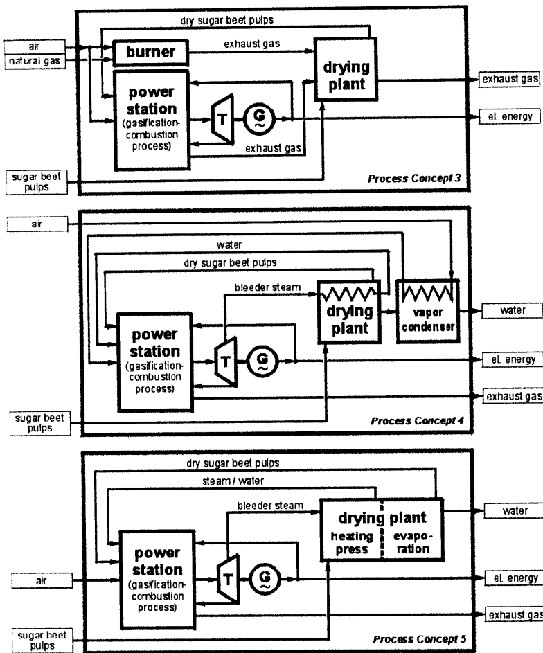
Figure 1b: Block flow diagrams for different energy utilizations of biomass in sugar industry (Concept 3, 4 and 5).
