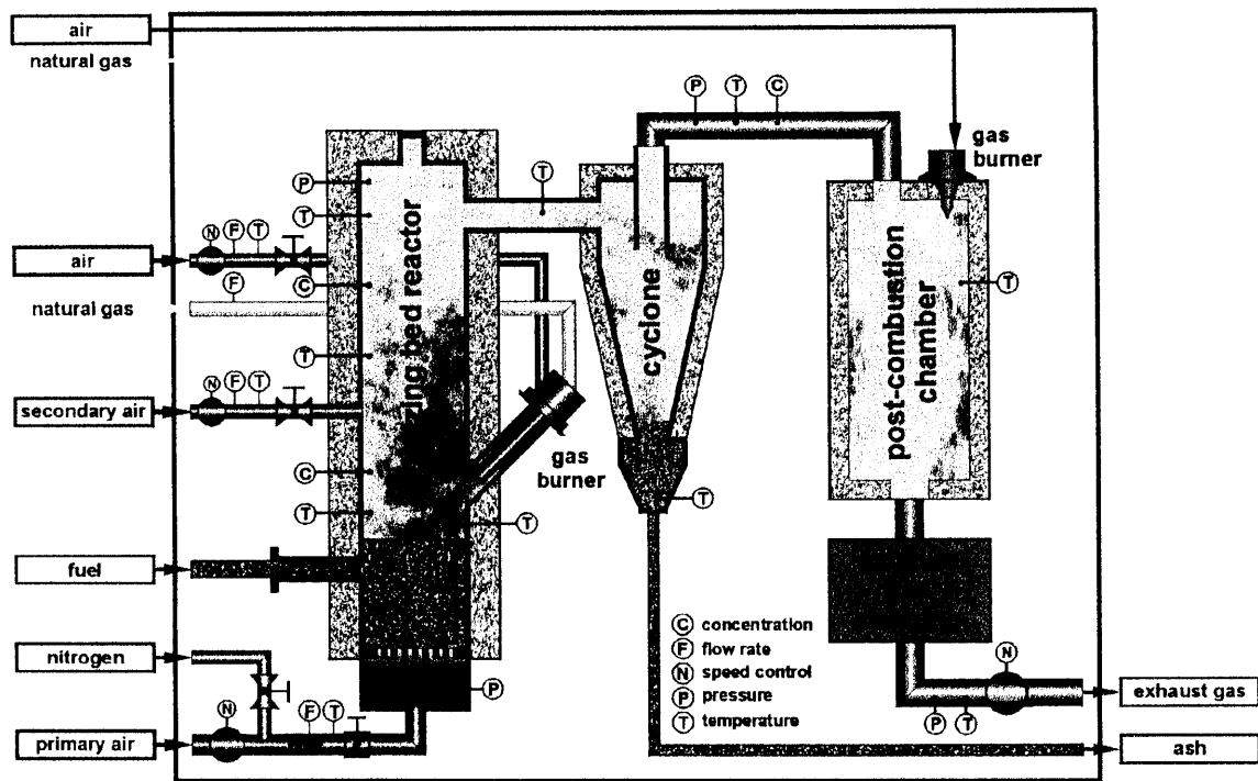
Figure 6: Flow chart of the fluidized bed reactor with post-combustion chamber.
