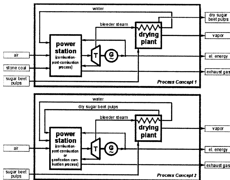
Figure 1a: Block flow diagrams for different energy utilisations of biomass in sugar industry (Concept 1 and 2).
