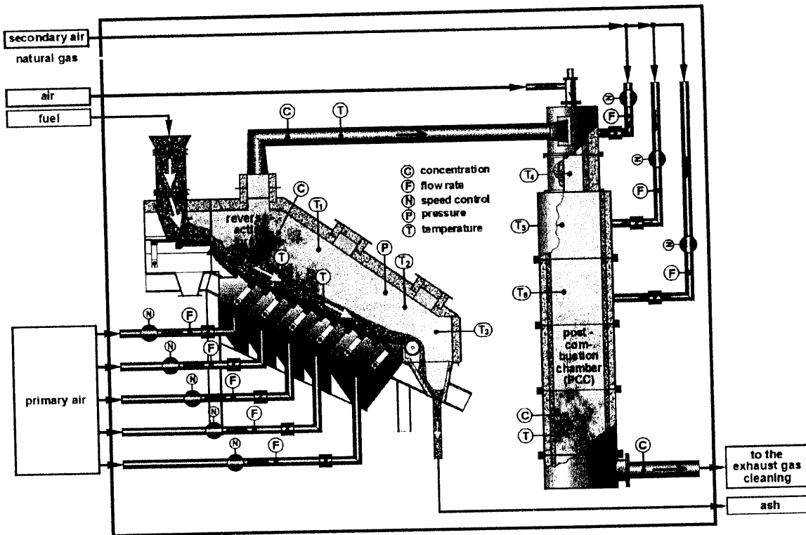
Figure 5: Flow chart of the reverse-acting grate system with a post-combustion chamber.
