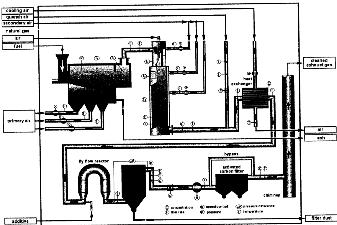
Figure 4: Flow chart of a forward-acting grate system (pilot plant) with post-combustion chamber and gas cleaning.
