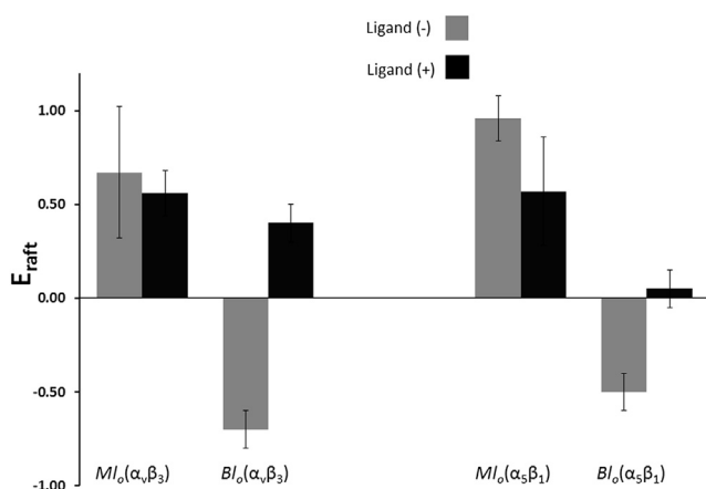
FIGURE 4 Comparison of E_{\text{raft}} values for \alpha_v\beta_3 and \alpha_5\beta_1 (with and without integrin ligands) as determined for bilayers with MI_o and Bl_o domains (light bars, -ligand; dark bars, +ligand).
